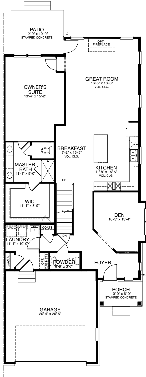
MAIN FLOOR
