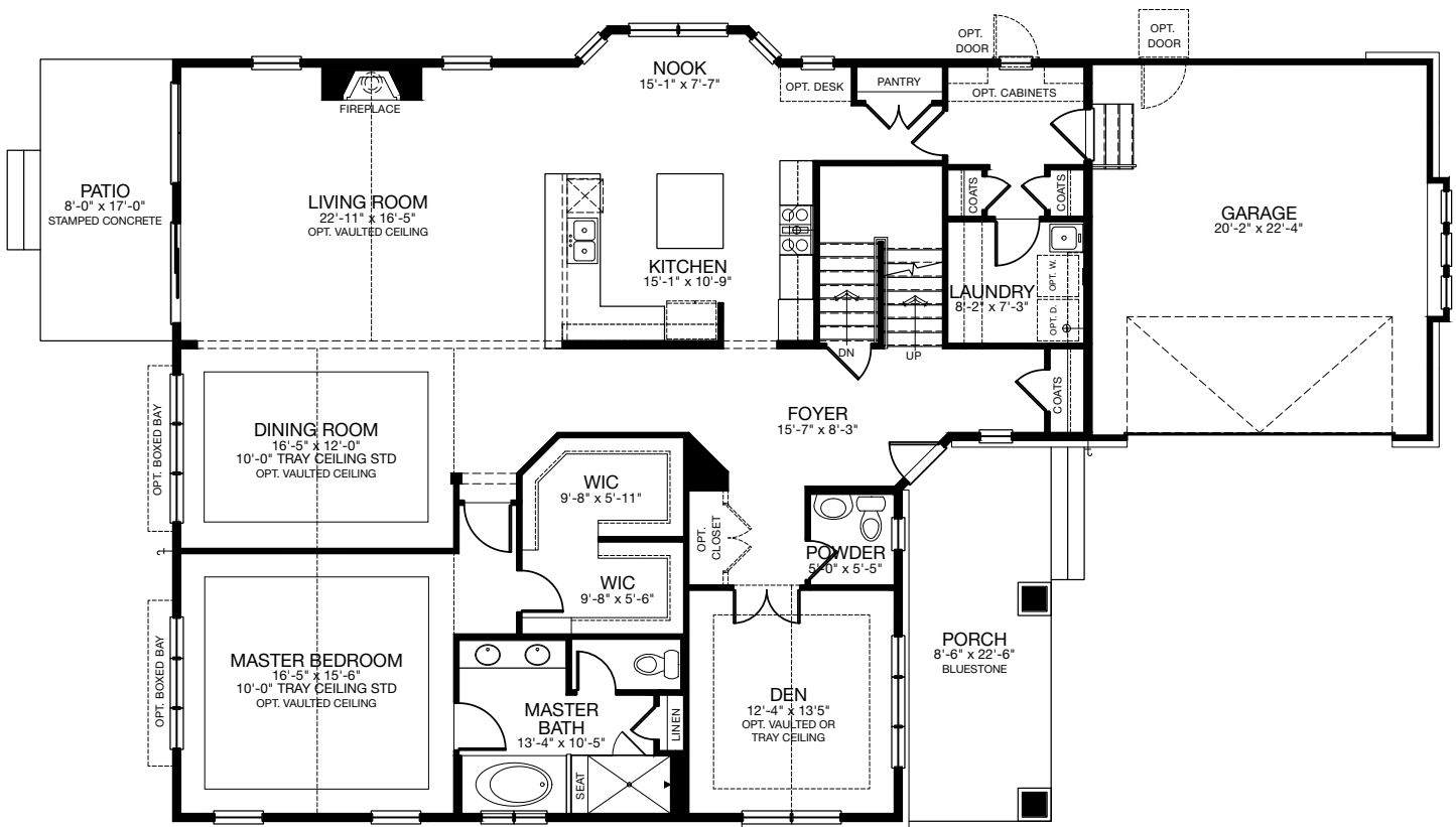
MAIN FLOOR COTTAGE
