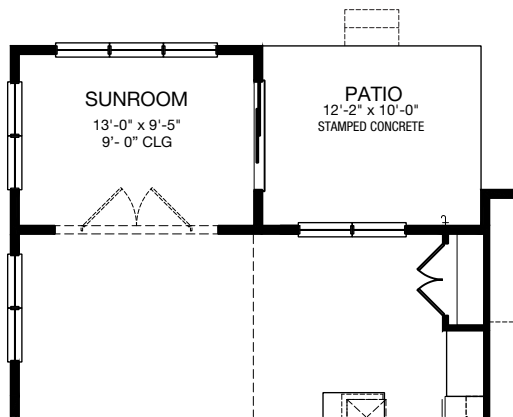
MAIN FLOOR OPTIONAL SUNROOM + 140 SF
