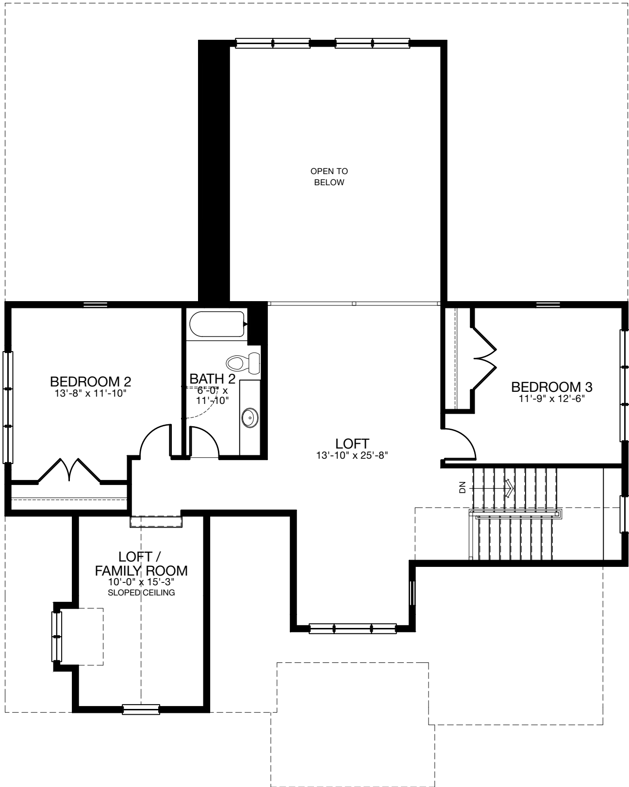
UPPER FLOOR COTTAGE
